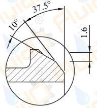
BUTTWELD END
