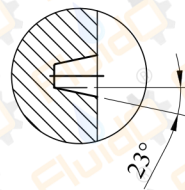
RTJ DETAILS
