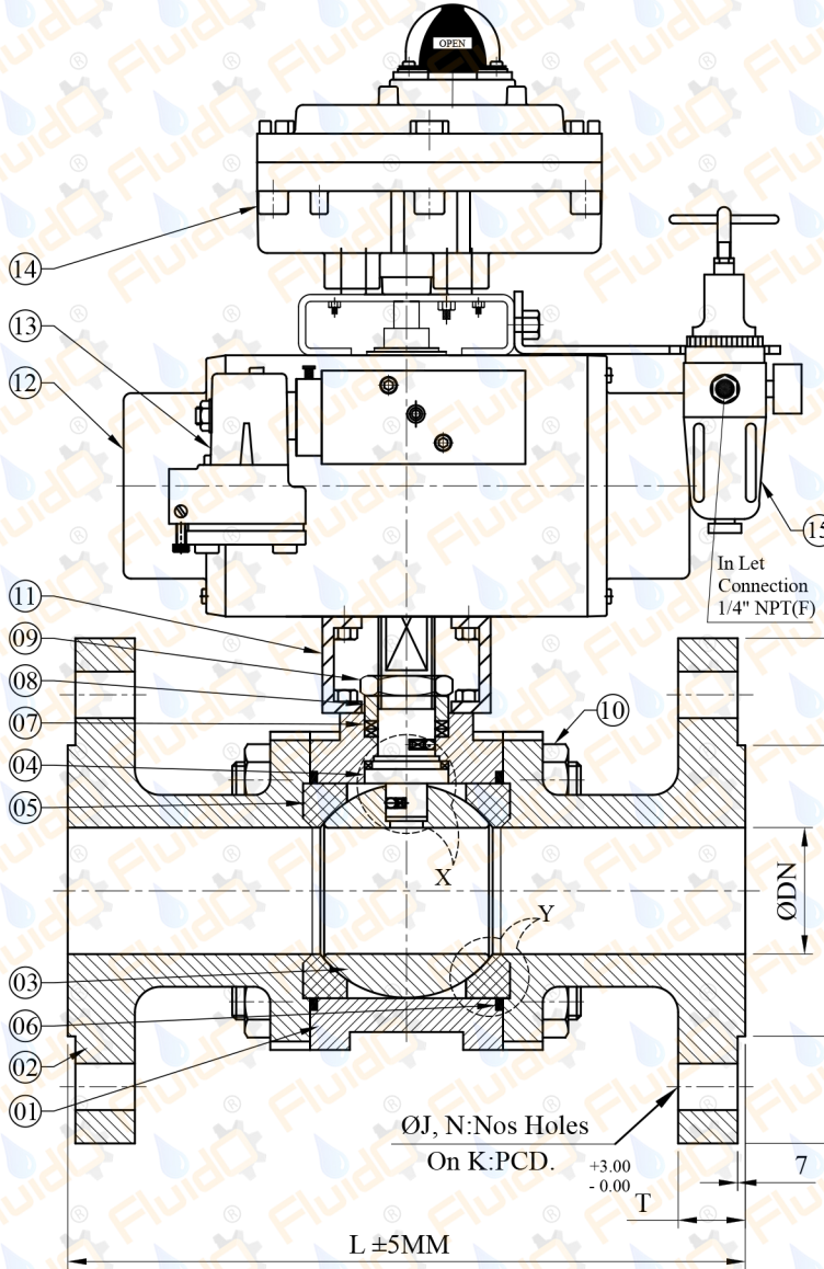
SECTIONAL ELEVATION
